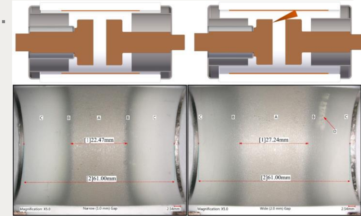
Controlling MVD by modifying Shield placements.
