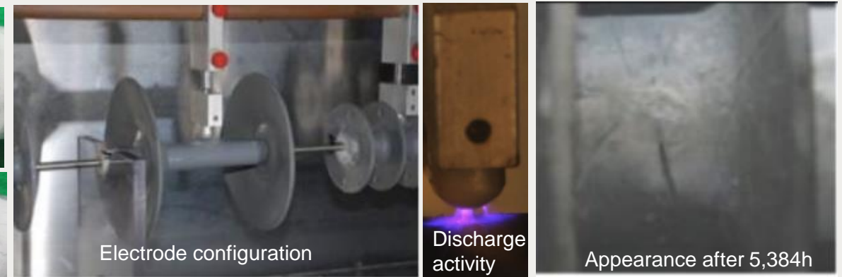
Fig. 5 Small-scale weathershed corona aging test developed by EPRI
