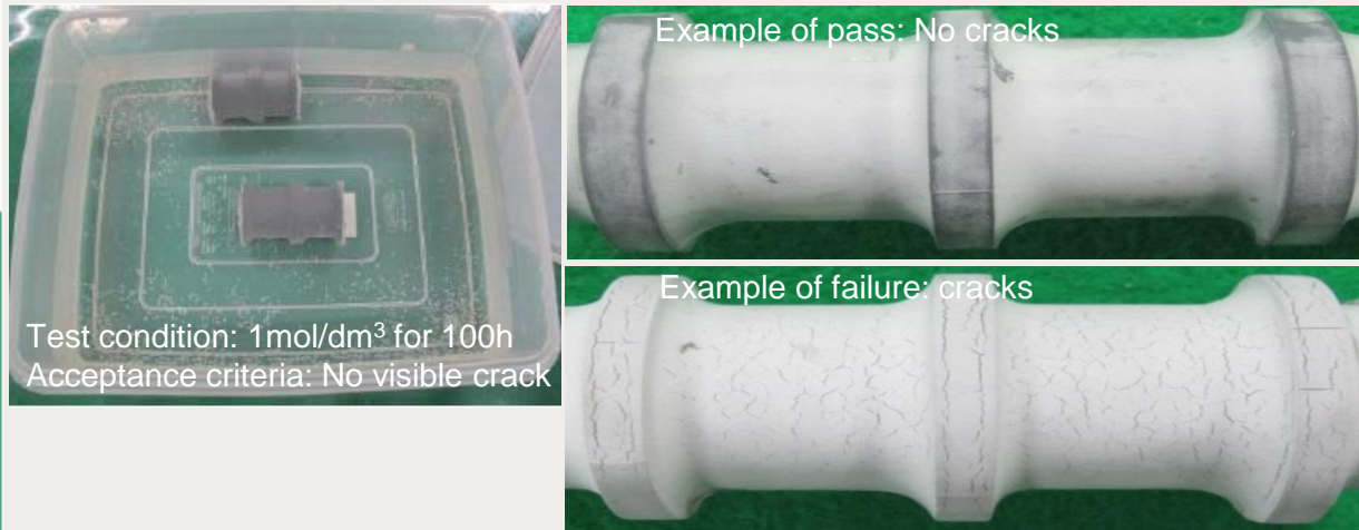
Fig.4 Nitric acid immersion test
