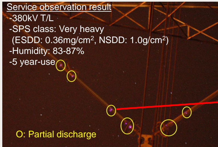
Fig.1 Partial discharge activity in service
