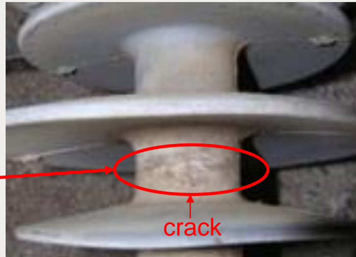
Fig. 2 Typical crack appearance on insulator trunk
