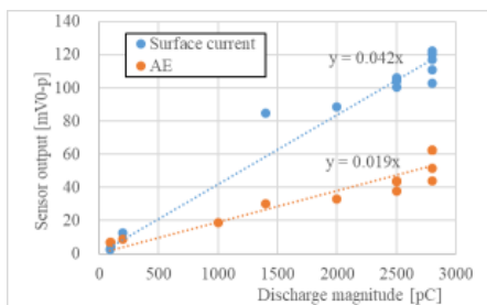
Figure 7 Experiment results of correlation between sensor output and amount of discharge
