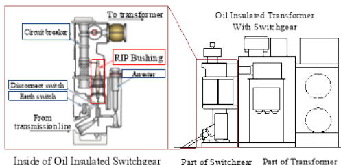
Figure 5 Application of resin bushings in oil insulated switchgear
