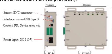
Figure 8 Appearance of stationary on-line PD monitoring device with automatic diagnosis
