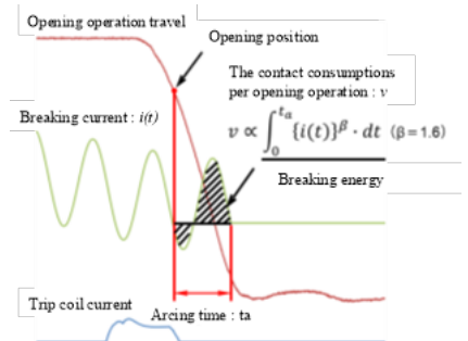
Figure 3 Method for calculating the contact consumption
