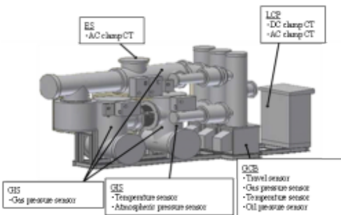
Figure 2 300 kV smart GIS sensor implementation
