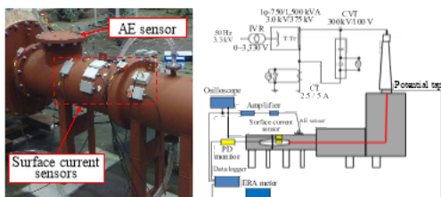
Figure 6 Construction of experimental system
